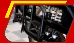
Suspension
